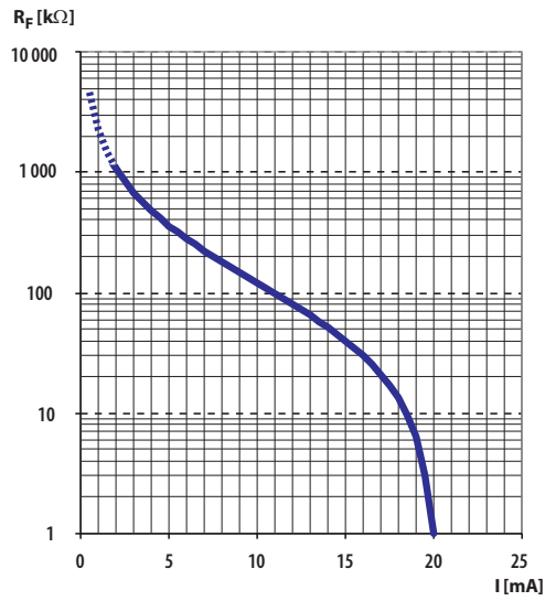
Stromausgang / Current output 0...20 mA
